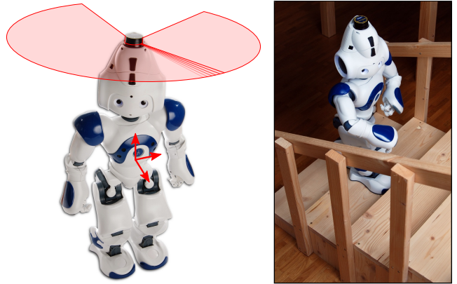
Fig. 1. Our laser-equipped Nao robot navigates in a multi-level indoor environment. The robot uses a head-mounted 2D laser range finder, attitude and joint angle sensors, as well as odometry information to perform Monte Carlo localization of its 6D torso pose while walking and climbing stairs.
