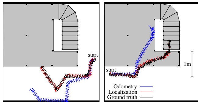
Fig. 6. Experiments carried out in our real-world environment (Left: ground floor only; right: ground floor and two stairs). Ground truth was obtained through a laser-based external tracking system. While odometry quickly diverges, our localization keeps track of the correct pose.
