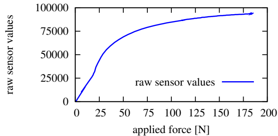
Fig. 3. Calibration data relating raw sensor values to forces calibrated using a load cell.
