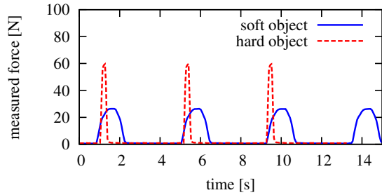
Fig. 5. Measured net fingertip force (N) for grasping a wooden block and a rubber toy when using a pure force controller. The high impact forces can destroy delicate, but rigid objects, like eggs.
