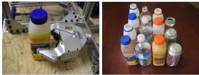
Fig. 4. Left: The experimental setup showing the gripper mounted on a stand. Right: Some of the bottles and cans used for our experiments. From left to right: Odwalla fruit juice bottle, water bottle, Naked fruit juice bottle, Coke can.
