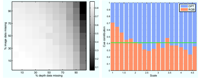
Fig. 4. Left: Graceful degradation of classification performance over ranges of invalid inputs. The diagram shows the F -score metric of the HGE fusion scheme with respect to missing data in each modality. Low F -score values are only caused by large amounts of missing information in both modalities. Right: Contribution of each modality to the final fused result. Blue bars represent the depth-based people detector contributions, red bars represent the vision-based detector contributions, with the green line being the average contribution over all scales. The visual detector has more importance at smaller scales when depth data are less reliable due to low signal-strength returns or out-of-range readings at far ranges.
