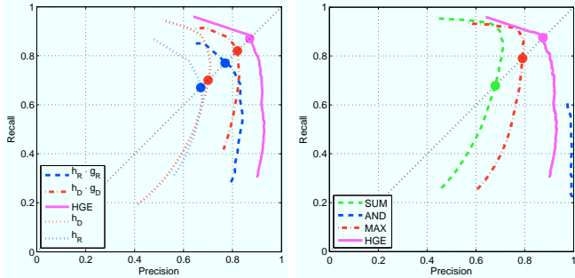
Fig. 3. Precision-recall curves for the Hierarchical Gaussian Process Mixtures of Experts approach (HGE). EER points are highlighted. Left: Classifier performance at places of increasing sophistication in the architecture in Fig. 1. The newly introduced gate functions g'(\cdot) have a clear contribution. Right: Comparison of alternative sensor fusion schemes including the proposed method (HGE), maximum detector response (MAX), product of detector responses (AND) and weighted sum of detector responses (SUM). HGE outperforms all other methods thanks to the adaptivity to the data conditions in each modality.
