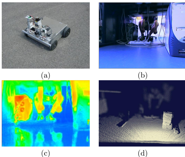
Fig. 1. The autonomous rescue robot Zerg (a) and vision data from the same scene (b)-(d): A color image taken by the CCD camera (b), a thermo image taken by the IR camera (c), and a 3D point set taken by the 3D scanner (d).
