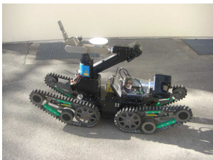
Figure 6. The teleoperated robot Telemax.
