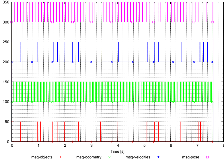
Figure 1. Recorded communication of the example robot control software. The peaks indicate the occurrence of the particular event.
