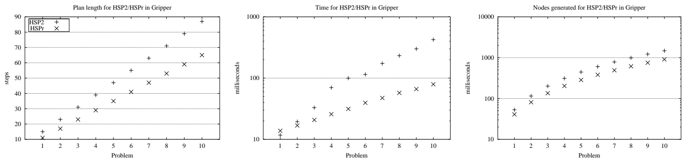
Figure 9: Comparison between HSPr vs HSP2 over Gripper instances. Curves show solution length (left), solution (center), and number of nodes generated (right)
