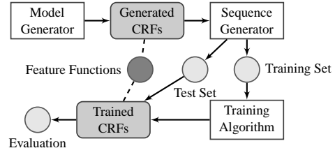
Figure 2: Training of CRFs with the shared features
