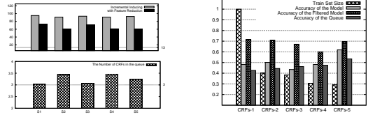
Figure 8: feature functions and CRFs in the queue Figure 9: An Example of CRF Queue
