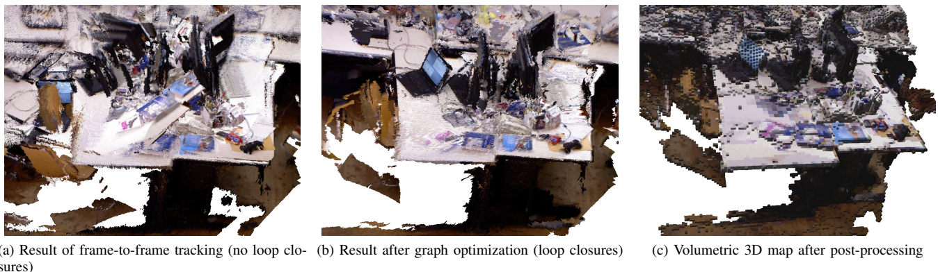
Fig. 3. (a) Using only stepwise tracking leads to undesired results due to the accumulated drift. (b) After graph optimization with 5 iterations of g^2o , an excellent alignment of most point clouds is achieved. Individual clouds are still slightly misaligned. (c) Through integration of the free-space information these artefact are greatly diminished after computation of occupancy probabilities.
