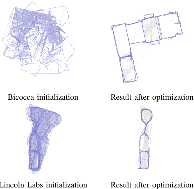
Fig. 3. Qualitative evaluation on 5 sessions of Bicocca (top) and 36 loops of Lincoln Labs (bottom) datasets that contain outliers generated by the vision system. Latif et al. [10] report a that RRR solves Bicocca in 314s whereas DCS requires only 1.56s to obtain the solution.
