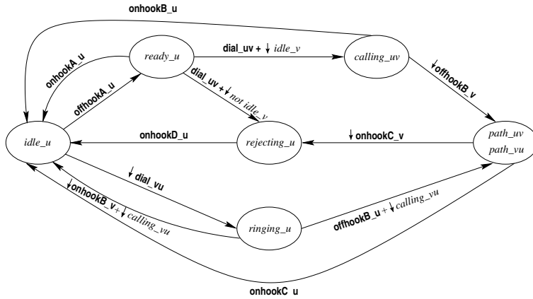
Figure 1: Transition system for a subscriber
