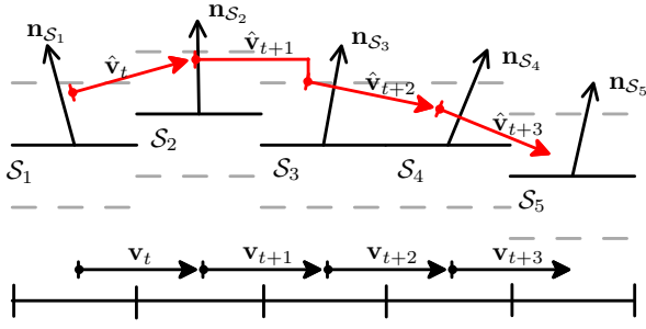
Fig. 2. Application of our prediction model to a series of 2D motion vectors (black). They are rotated to estimate the 3D motion vectors (red). The dashed line indicates the tolerance interval for the z -coordinate.
